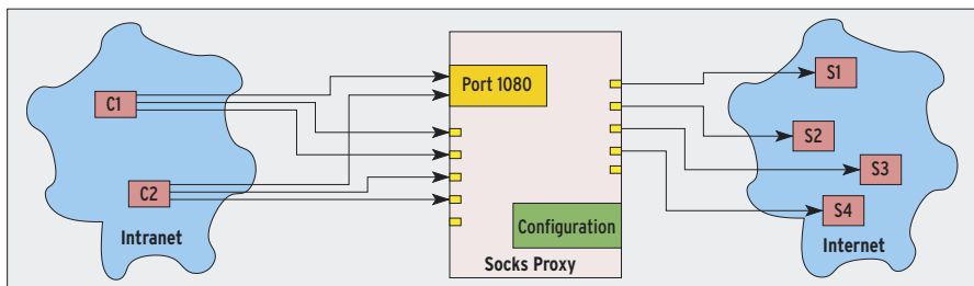
Figure 1b: In contrast to an ALG, Socks assumes the role of a generic proxy, accepting connections for any application protocols on port 1080, authenticating clients, and authorizing transfers.
